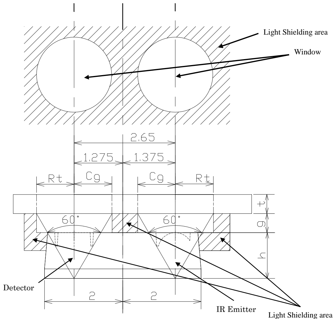
GP2AP030A00F
