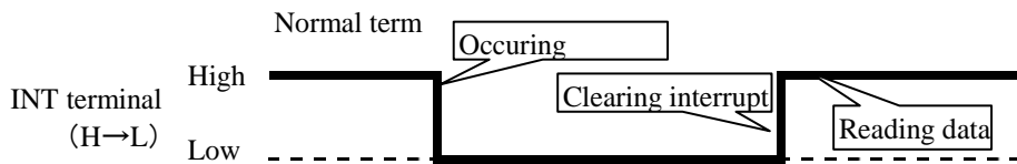
Fig.14 Interrupt output (level interrupt type)
