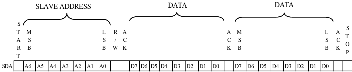
Fig.2 I 2 C Basic data format
