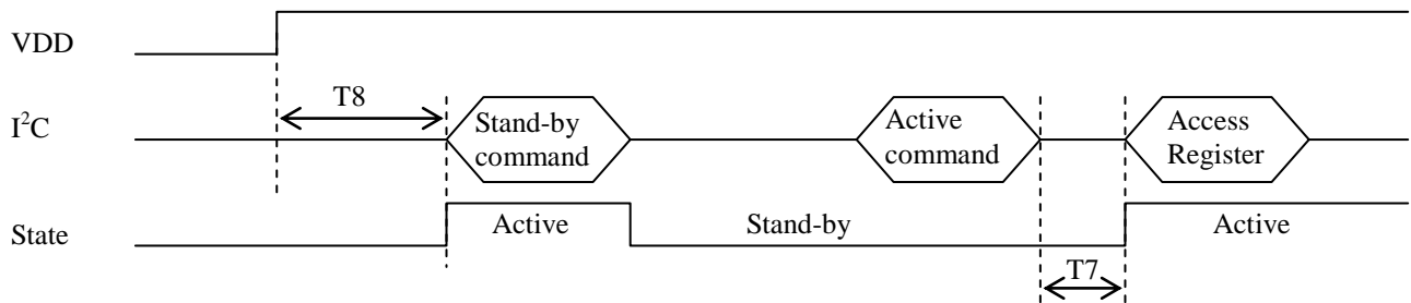
Fig.03(a) Timing chart of active/stand-by state control (GP2Y0E02B)
