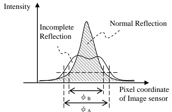
Fig.32 Spot size of incomplete and normal reflection
