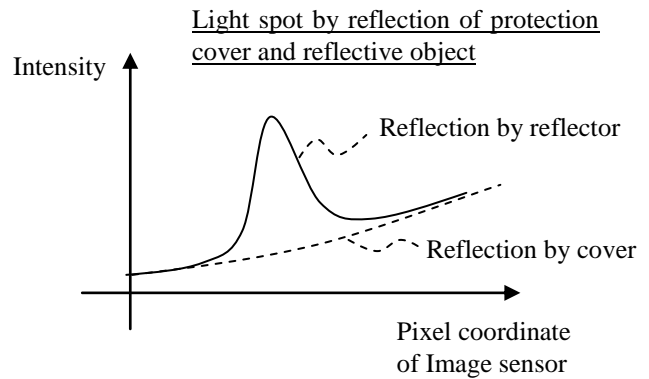
Fig.24 light spot profile of cover and reflective object
