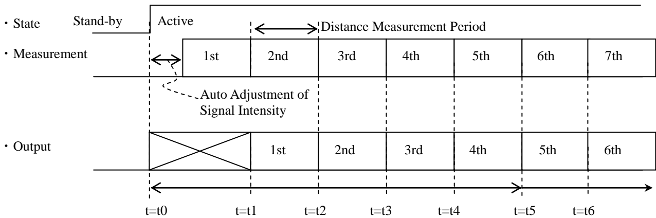
Fig.22 Median Filter
