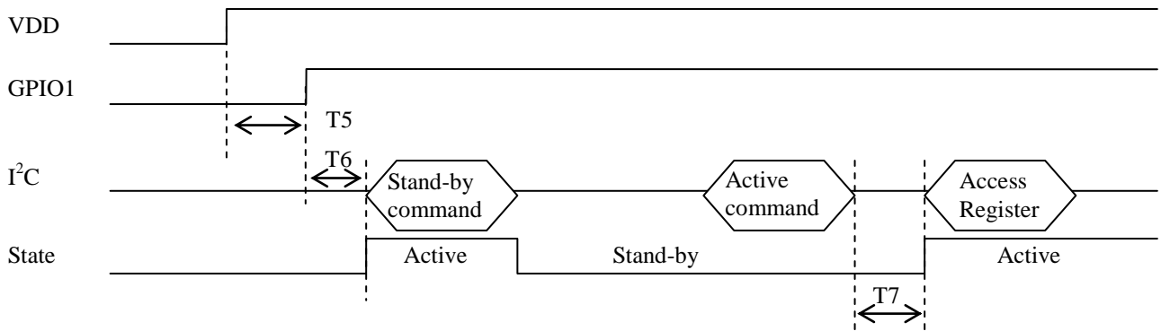
Fig.03(a) Timing chart of active/stand-by state control (GP2Y0E02A)
