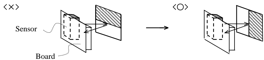
Fig.08 Recommended measurement of reflective object with boundary line
