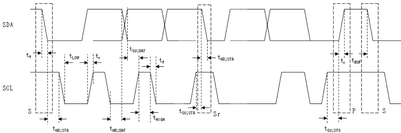
Fig.20 I 2 C Bus Timing
