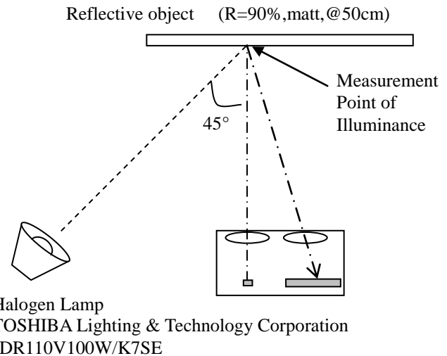
Fig.18 Apparatus of ambient light characteristic measurement
