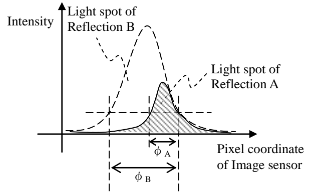
Fig.31 Spot size of partial and whole reflection
