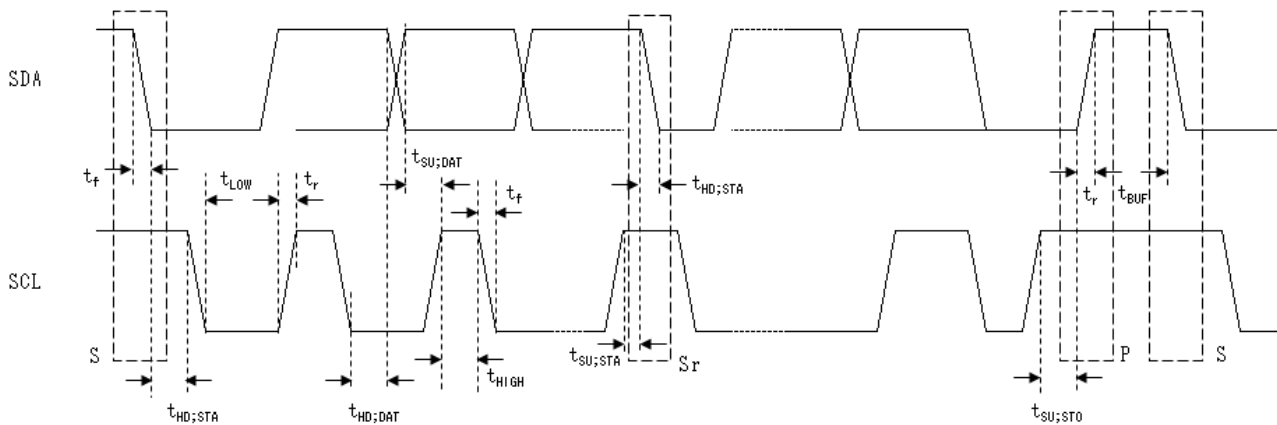
Fig.20 I 2 C Bus Timing
