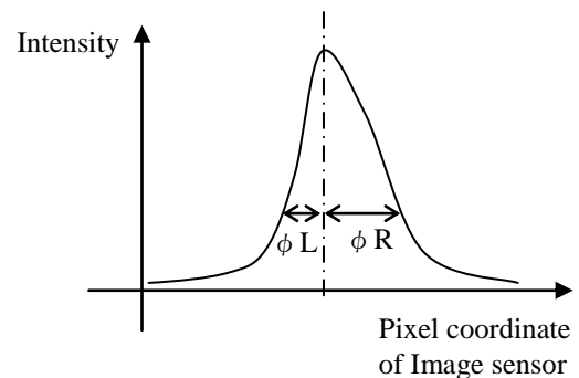
Fig.33 Asymmetric Light Spot
