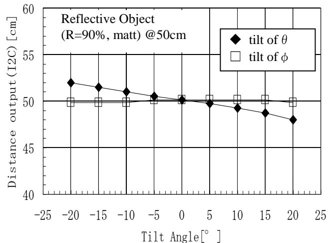
Fig.14 Tilt Angle Dependence of distance output
