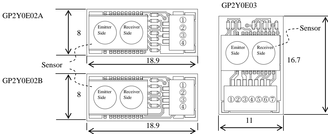
Fig.01 Outline of GP2Y0E series
