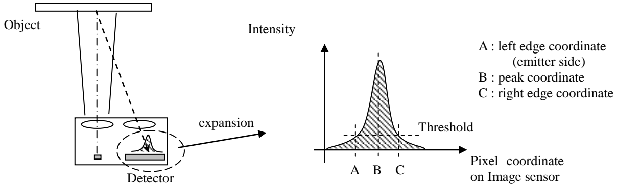
Fig.21 Coordinate of spot profile
