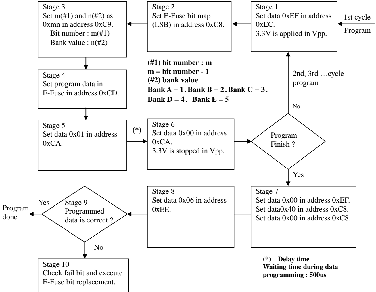
Fig.40 E-Fuse Program Flow
