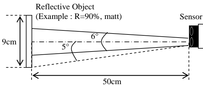
Fig.09 Reflective Object Size
