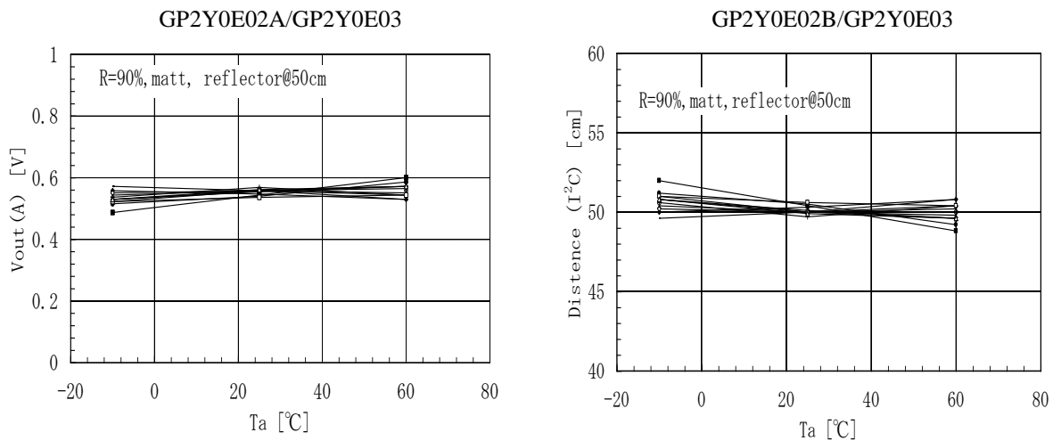
Fig.17 Example of ambient temperature characteristic
