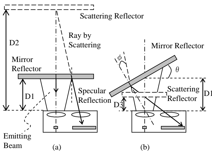
Fig.05 Mirror Reflector
