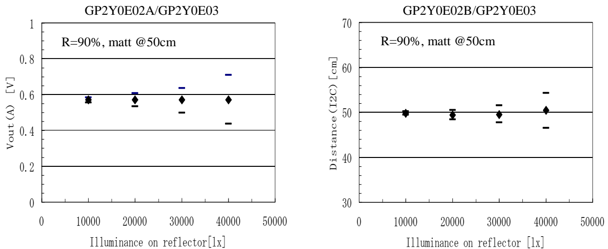
Fig.19 Ambient Light Characteristic
