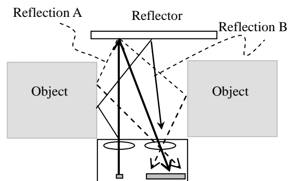
Fig.06 Case that object is near the sensor
