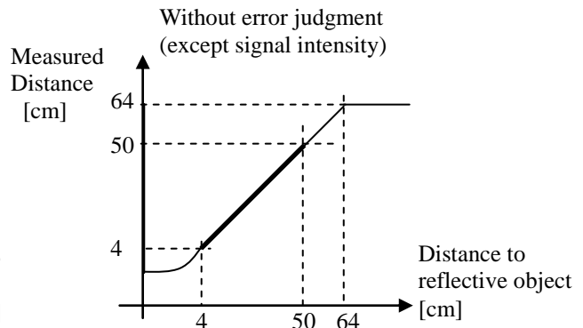
Fig.35 Distance characteristic without error judgment
