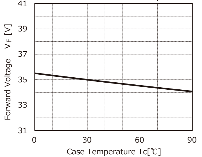
Case Temperature vs. Forward Voltage
